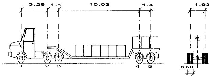
Fig. 3 : Configuration of SCANIA Truck
