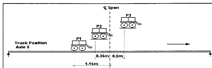
Fig. 5 : Typical Truck's Longitudinal Load Positions
