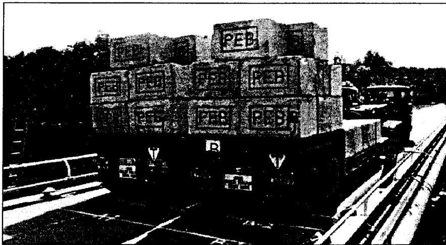
Fig.6 : Two trucks carrying maximum loads during load testing
