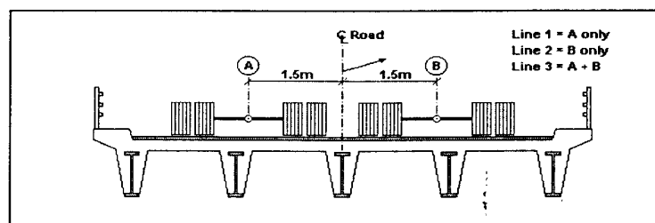
Fig. 4 : Typical Truck's Transverse Position
