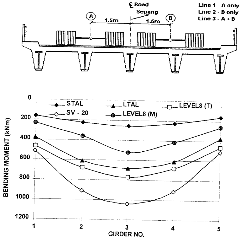
Fig. 7 : Comparison of Moment Induced by Various Loadings
