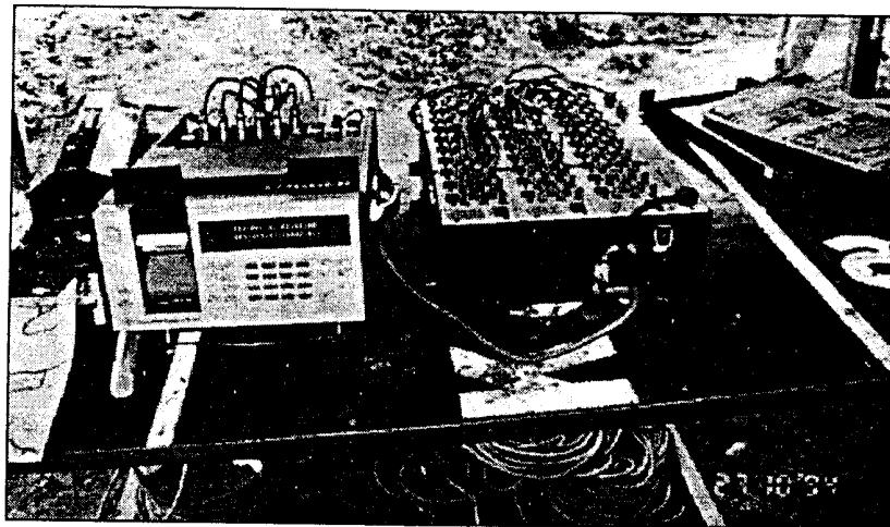
Fig. 2 : Data Acquisition using a data logger and a 20 channel multiplexor
