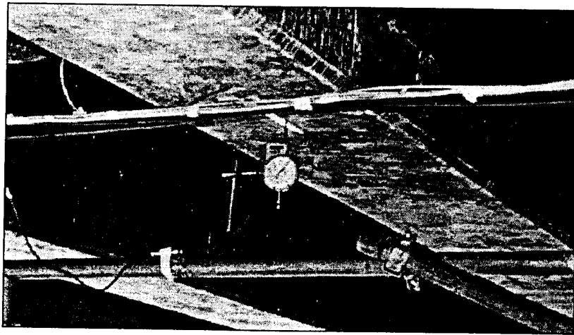
Fig 1 : Instrumentation of r.c. beam using strain and dial gauges
